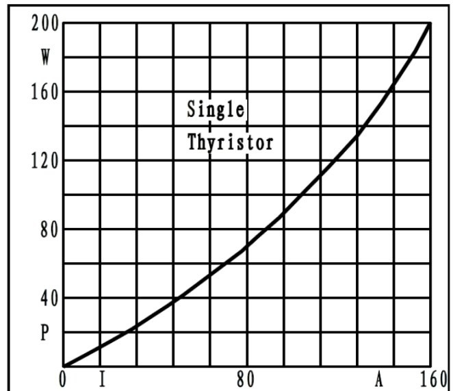
Fig3. Power dissipation
